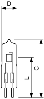
EcoHalo Capsule Gy6.35 12v14w CL B3000
