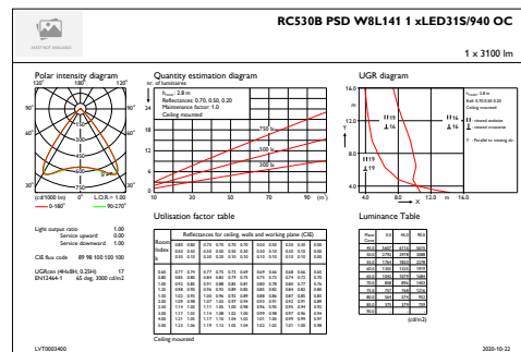
IFGU1_RC530BPSDW8L1411xLED315940OC
