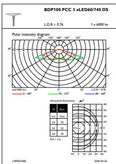
OFPL1_BDP100PCC1xLED60740DS
