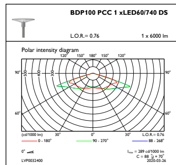
OFPC1_BDP100PCC1xLED60740DS
